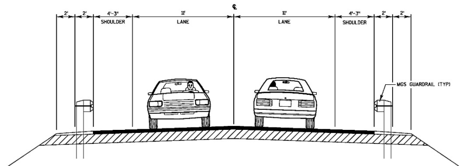
TYPICAL FINISHED SECTION CTH V W/GUARDRAIL
