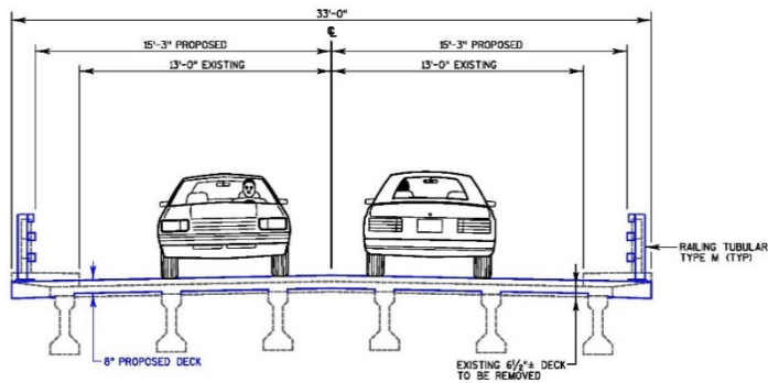
TYPICAL FINISHED SECTION CTH V THRU BRIDGE
